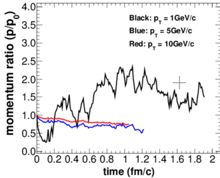
Figure 3. (Color Online) Energy loss of heavy quarks with different initial momentum as a function of time. The parameters of this figure is the same with Figure 2.
