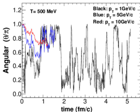
Figure 4. (Color Online) Time evolution of the angular between charm c and anti-charm \bar{c} quark momentum in the deconfined medium in proton-proton collisions. Medium temperature is now taken as 0.5 GeV, where charm quarks can be thermalized easily, and the angular between c and \bar{c} becomes random when they move out of the hot medium.
