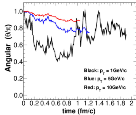
Figure 2. (Color Online) Time evolution of the angular between charm c and anti-charm \bar{c} quark momentum in the deconfined medium produced in proton-proton collisions. Charm and anti-charm quark momentum is taken as 1, 5, 10 GeV/c respectively, with opposite direction. Deconfined medium temperature is taken as a constant typical value of T_{QGP} = 0.3 GeV. The parameter indicating the coupling strength between heavy quark and the bulk medium is taken as C = 1 .
