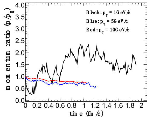
Figure 3. Energy loss of heavy quarks with different initial momentum as a function of time. The parameters of this figure is the same with Figure 2.
