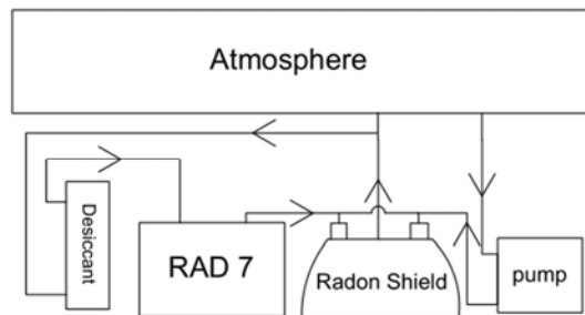
Figure 1. Radon Exhalation Rate Measuring Device.
