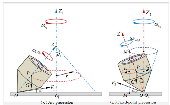
Figure 7. The rotation axis sweeps through the conical surface in the precession process of gyro.
